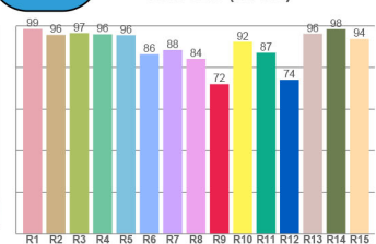
CRI: 92.6 (R1-R8)
